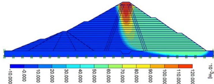
Figure 15. Possible failure surface of clay core embankment dam (by shading approach) (source: Plaxis Output).
