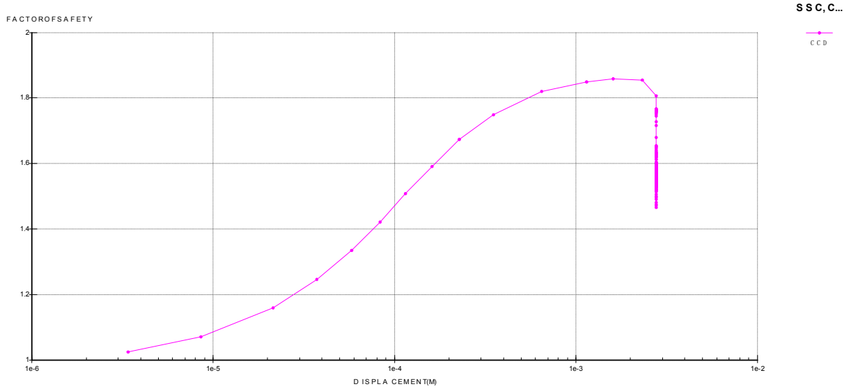
Figure 12. Factor of Safety of Clay Core embankment dam (steady-state condition) (source: Plaxis Output).
